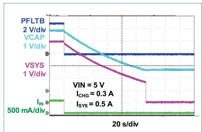
Figure 6 : Discharging Time (SuperCap1 = SuperCap2 = 20 F)
