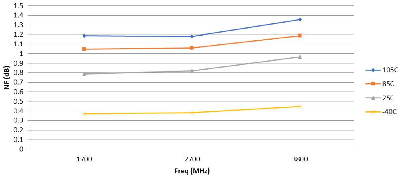
GRF4014 Evaluation Board Noise Figure vs. Frequency vs. Temperature; Vdd: 5.0 volts
