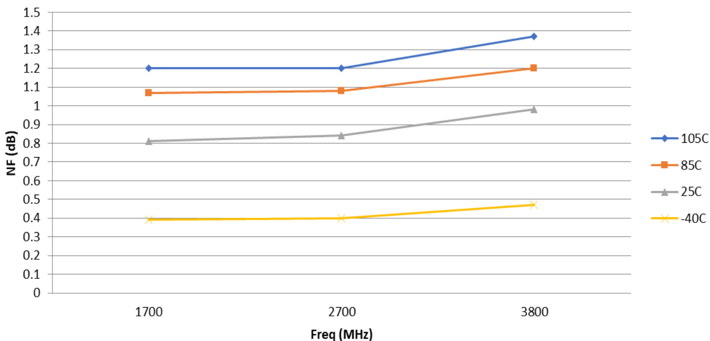
GRF4014 Evaluation Board Noise Figure vs. Frequency vs. Temperature; Vdd: 8.0 volts
