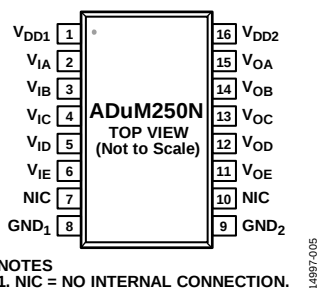
Figure 5. ADuM250N Pin Configuration
