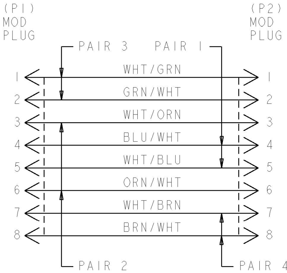
WIRING DIAGRAM 568A
