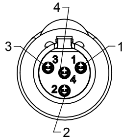
TA4FS SERIES 4 PIN
