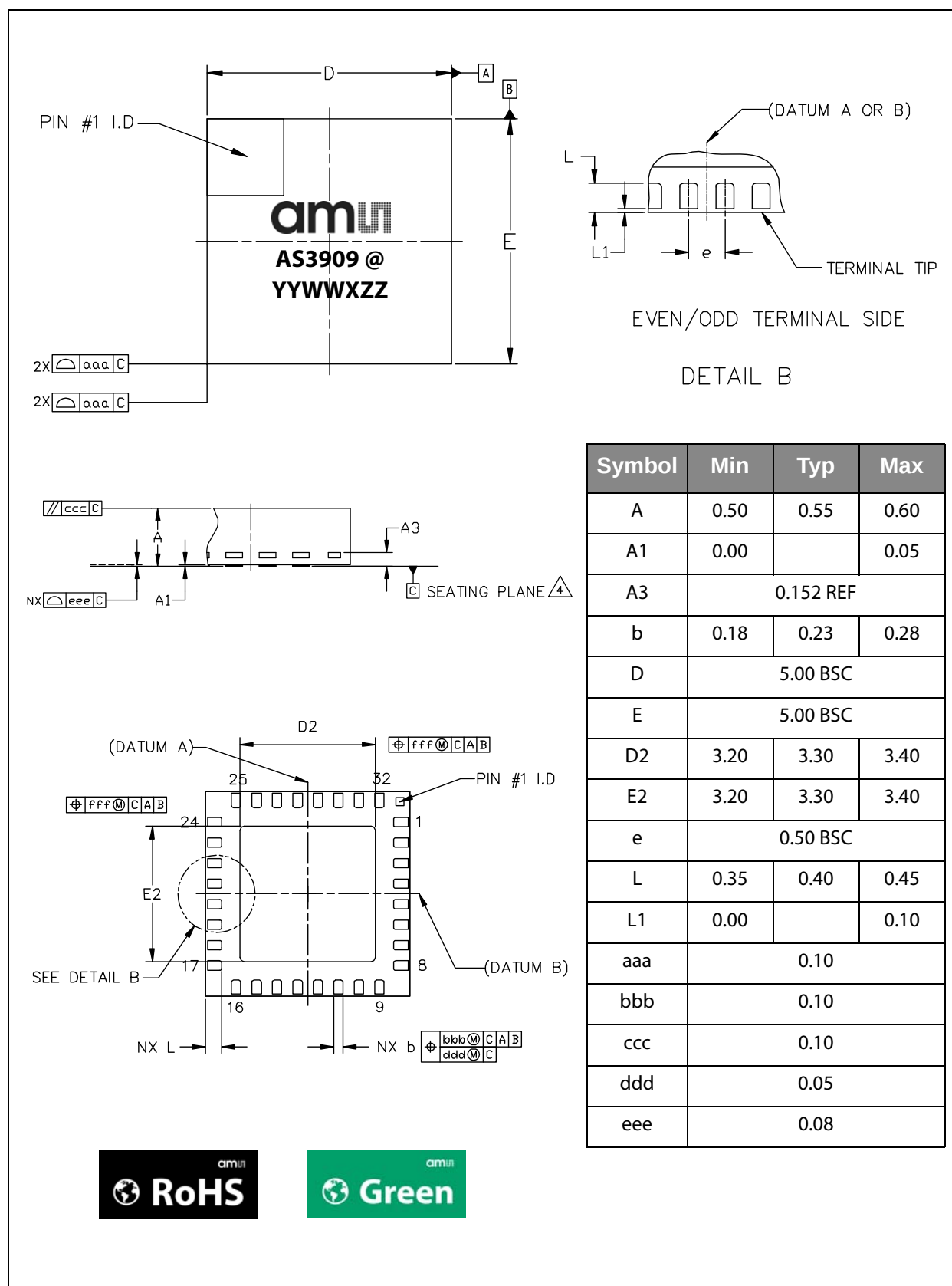
Figure 54: Package Drawings for AS3909 (TQFN)
