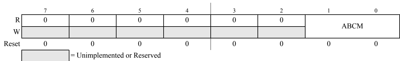
Figure 6-4. Debug Control Register2 (DBGCI2)
