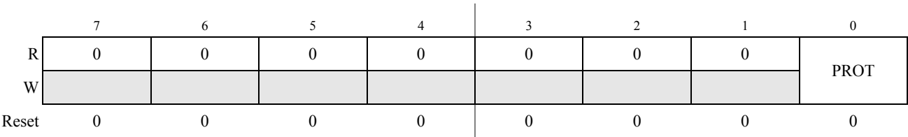
Figure 8-32. S12CPMU_UHV_V7 Protection Register (CPMUPROT)
