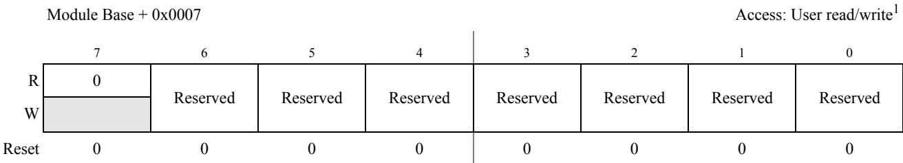
Figure 19-5. Reserved Registerfv_dac_8b5v_RESERVED
