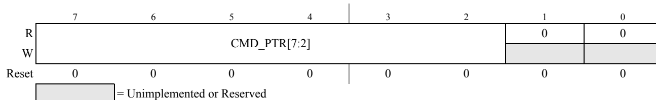
Figure 9-23. ADC Command Base Pointer Registers (ADCCBP_0, ADCCBP_1, ADCCBP_2))
