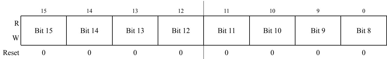
Figure 11-22. Timer Input Capture/Output Compare Register x High (TCxH)
