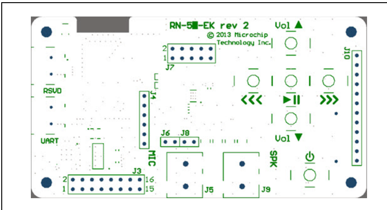
FIGURE A-2: RN52 EVALUATION BOARD TOP SILKSCREEN
