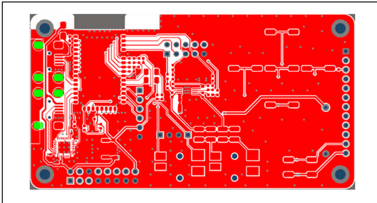
FIGURE A-4: RN52 EVALUATION BOARD TOP COPPER
