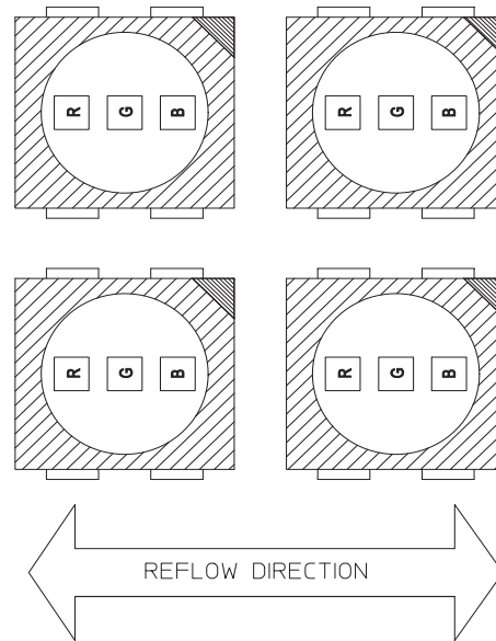
Figure 16: Recommended Board Reflow Direction
