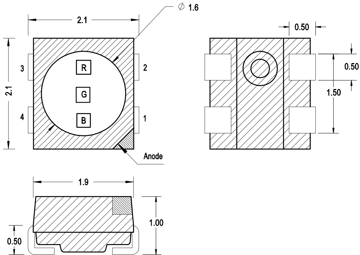
Figure 1: Package Drawing
