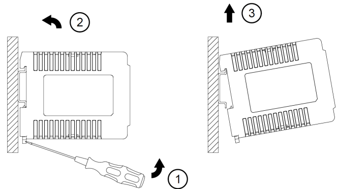
Fig. 2.2 Dismounting
