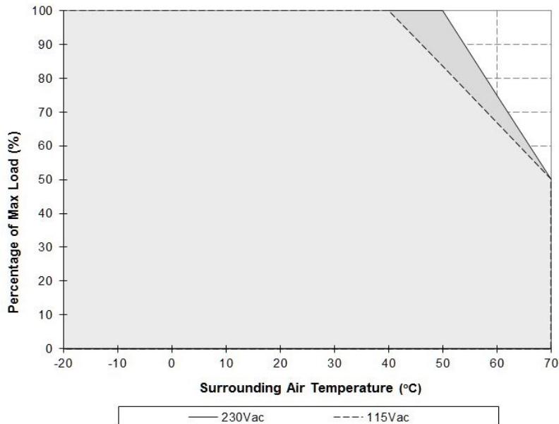
Fig. 1 De-rating for Vertical Mounting Orientation > 40°C de-rate power by 1.67% / °C @ 115Vac (Test at 115Vac condition) > 50°C de-rate power by 2.5% / °C @ 230Vac (Test at 230Vac condition)
