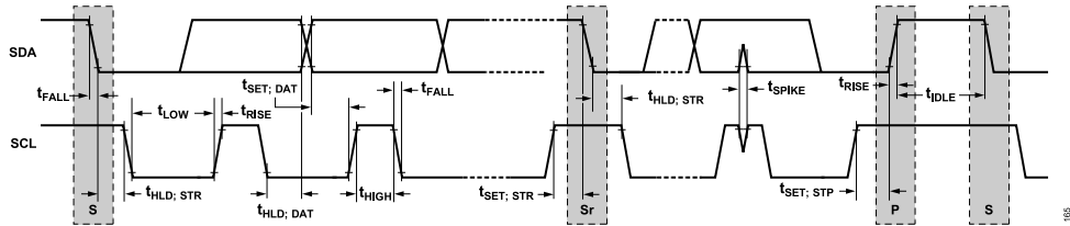
Figure 35. I 2 C Serial Port Timing
