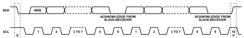
Figure 32. Acknowledge Bit
