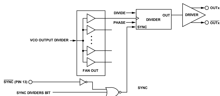
Figure 27. Clock Output Synchronization Block Diagram
