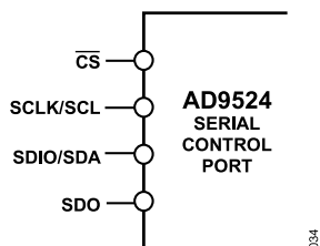
Figure 36. Serial Control Port
