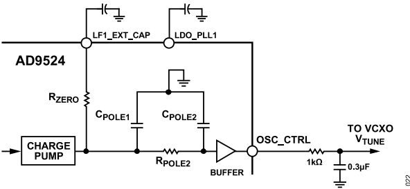
Figure 23. PLL1 Loop Filter
