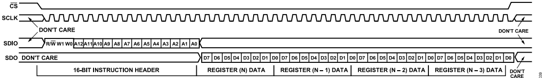
Figure 40. Serial Control Port Read—MSB First, 16-Bit Instruction, Four Bytes of Data
