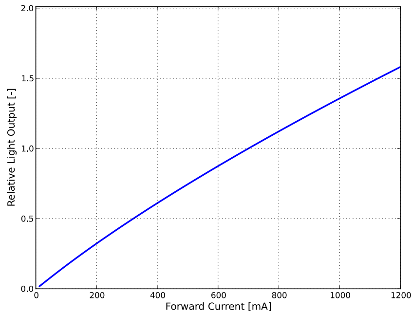
Figure 3a: Typical normalized light output vs. forward current for LMZx-Sxxx at T j =85°C.
