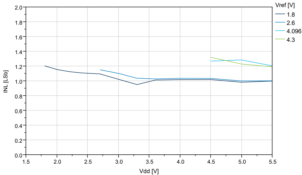
Figure 5-58. INL vs. V_{DD} ( f_{ADC}=115 kps, T=25^{\circ}C , REFSEL = External Reference)
