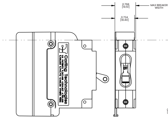
1-POLE (CA1) W/ ARC CHUTE BARRIER
