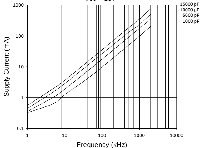
Fig. 12 Supply Current vs. Frequency V CC = 18V
