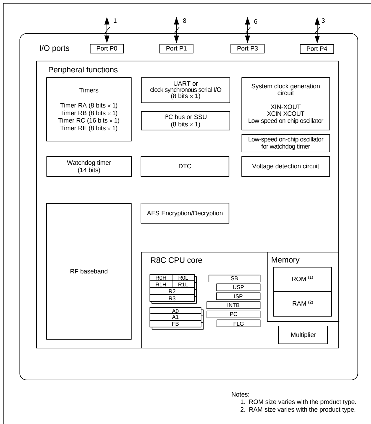
Figure 1.2 Block Diagram
