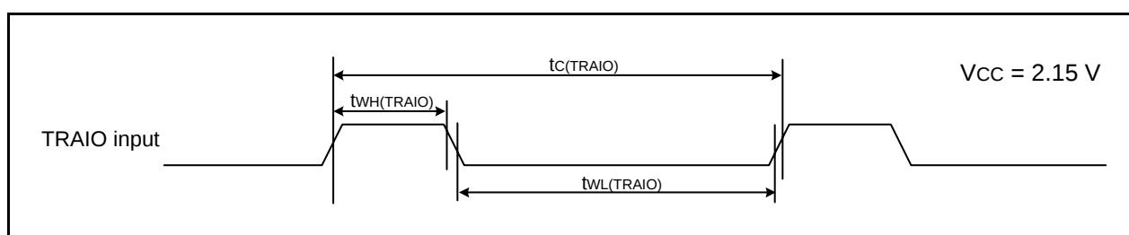
Figure 5.11 TRAIO Input Timing Diagram when V_{CC} = 2.15\text{ V}
