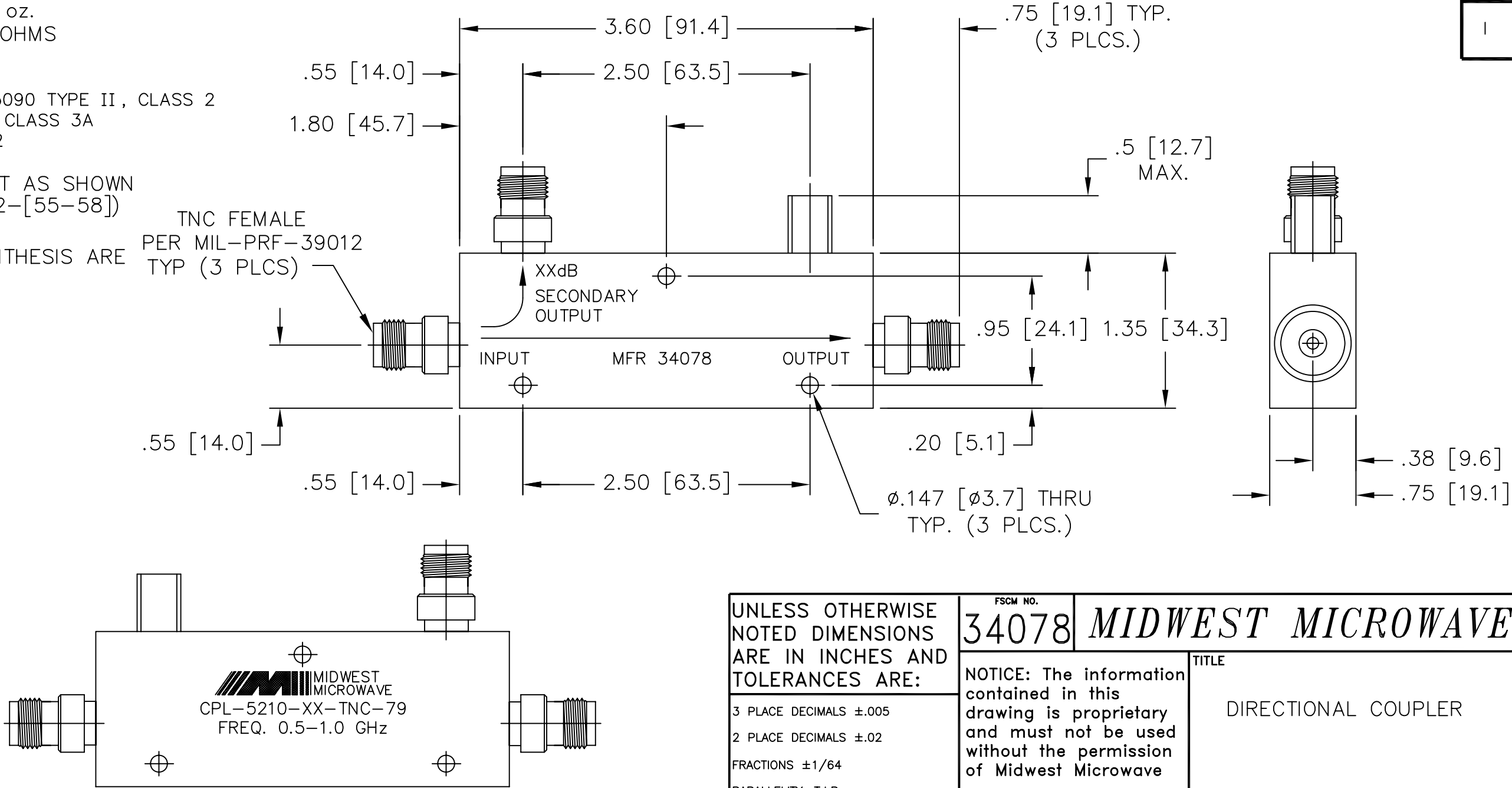
BACKSIDE MARKING
