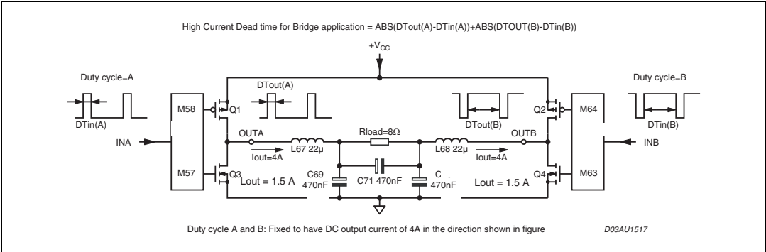
Figure 5. Test circuit
