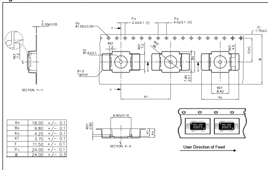
Figure 37. Reel information
