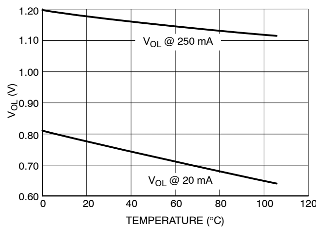
Figure 13. Driver 2 Output Voltage Low State @ V_{CC} = 15\text{ V} vs. Temperature
