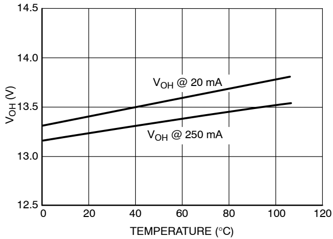
Figure 10. Driver 1 Output Voltage High State @ V_{CC} = 15\text{ V} vs. Temperature
