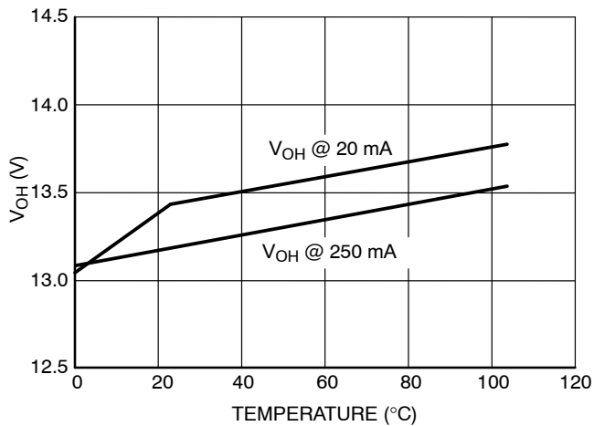
Figure 12. Driver 2 Output Voltage High State @ V_{CC} = 15\text{ V} vs. Temperature
