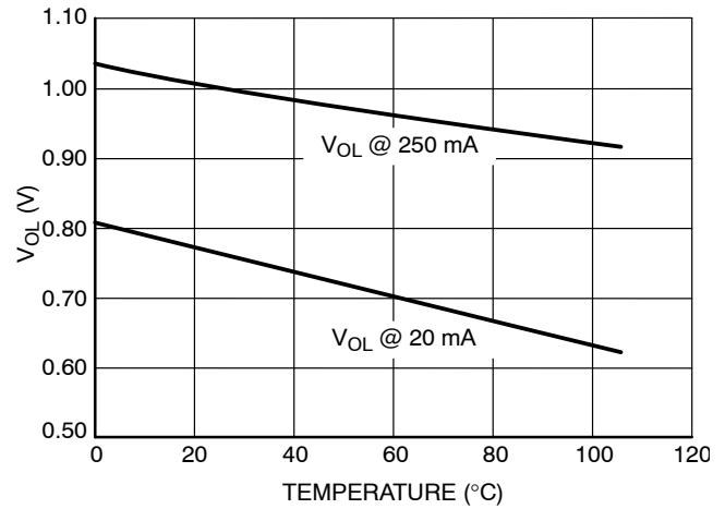
Figure 11. Driver 1 Output Voltage Low State @ V_{CC} = 15\text{ V} vs. Temperature
