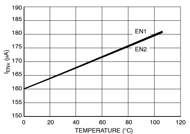
Figure 15. Soft-Start Current Source on Enable Pin when V_{ENx} = 2.5\text{ V} vs. Temperature
