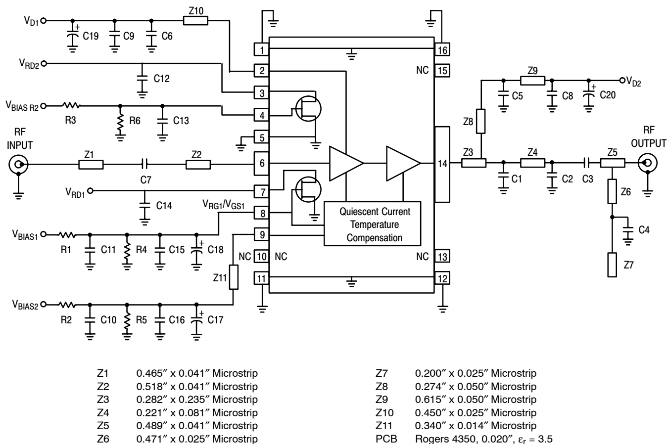
Figure 22. MW5IC2030NBR1(GNBR1) Test Circuit Schematic for Driver Application Tests
