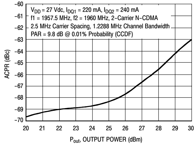
Figure 24. 2-Carrier N-CDMA ACPR versus Output Power
