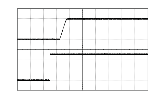
Start-up by enabling CTRL signal at: T_{P1} = +25\text{ }^\circ\text{C} , V_i = 12\text{ V} , V_o = 1.0\text{ V} C_o = 470\text{ }\mu\text{F}/10\text{ m}\Omega , I_o = 25\text{ A} Top trace: output voltage (0.5 V/div.). Bottom trace: CTRL signal (2 V/div.). Time scale: (20 ms/div.).
