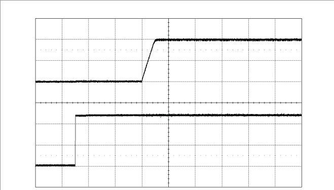
Start-up enabled by connecting V_i at: T_{P1} = +25\text{ }^\circ\text{C} , V_i = 12\text{ V} , V_o = 1.0\text{ V} C_o = 470\text{ }\mu\text{F}/10\text{ m}\Omega , I_o = 25\text{ A} Top trace: output voltage (0.5 V/div.). Bottom trace: input voltage (5 V/div.). Time scale: (20 ms/div.).
