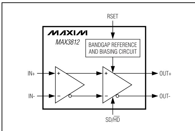
Figure 2. Functional Diagram
