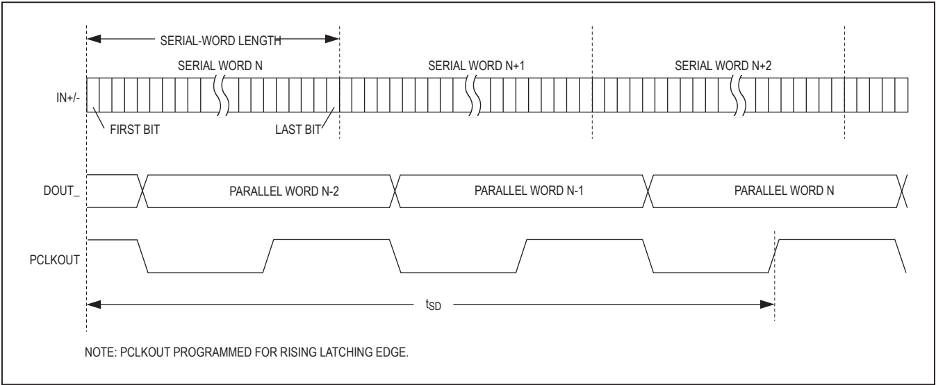
Figure 7. Deserializer Delay
