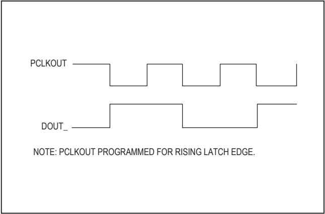
Figure 3. Worst-Case Pattern Output
