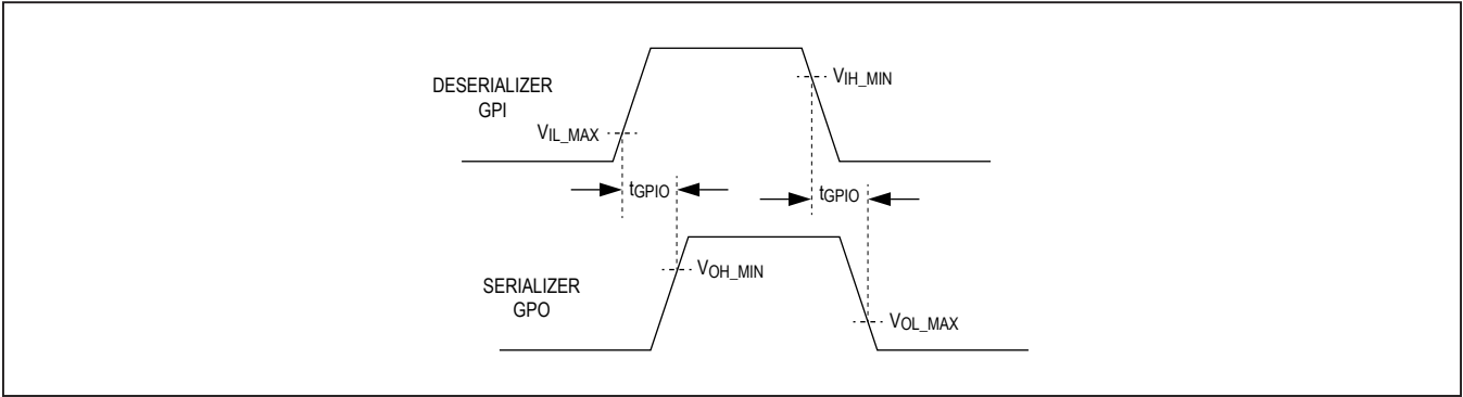
Figure 8. GPI-to-GPO Delay
