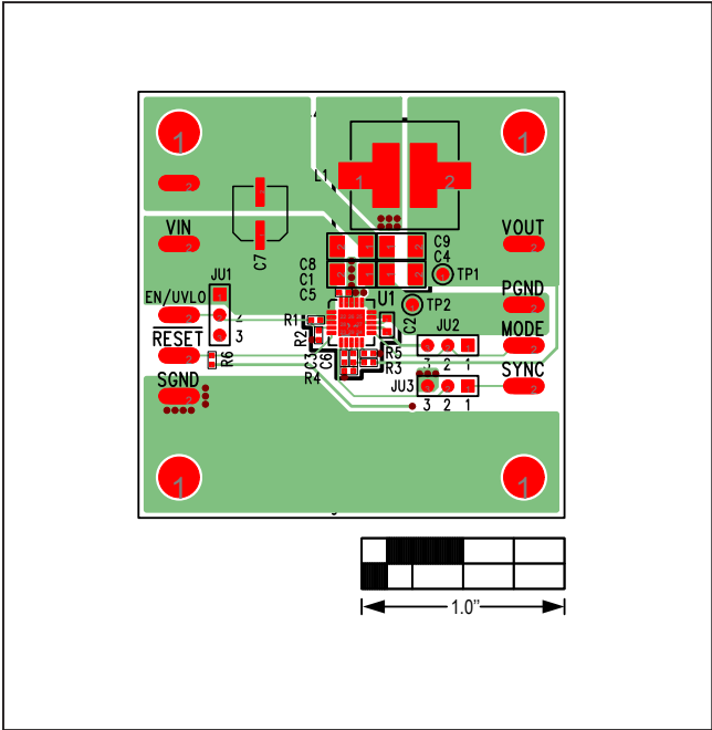
Figure 13. MAX17544 5V Output EV Kit Component Side PCB layout
