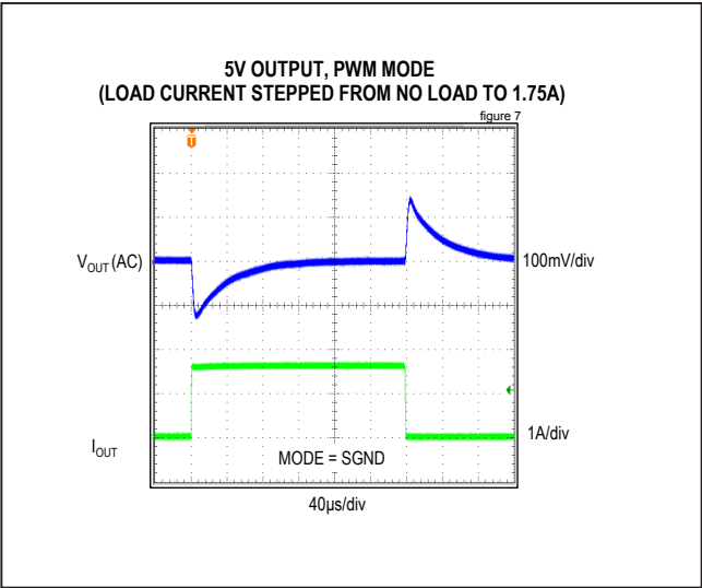
Figure 7. MAX17544 5V Output, No Load to 1.75A Load Transient (PWM Mode)
