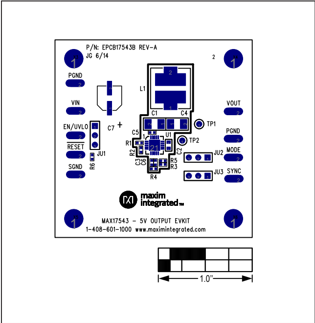
Figure 12. MAX17543 5V Output EV Kit Component Placement Guide—Component Side
