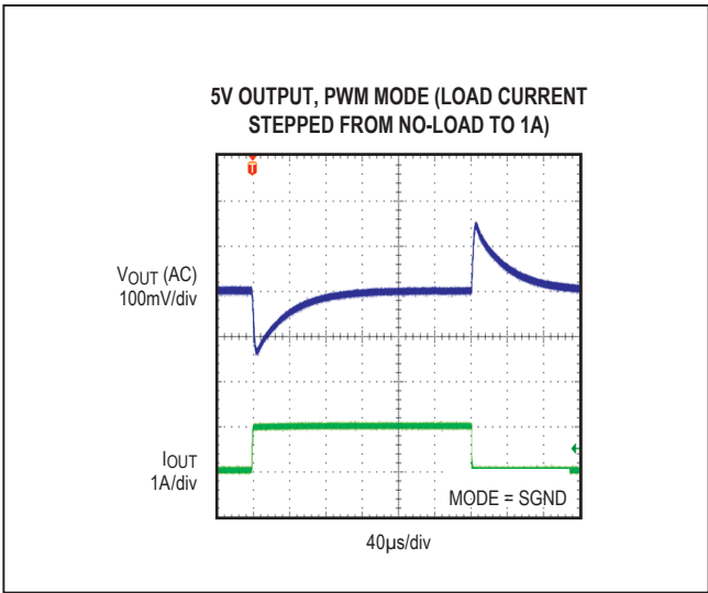
Figure 7. MAX17543 5V Output, No Load to 1A Load Transient (PWM Mode)
