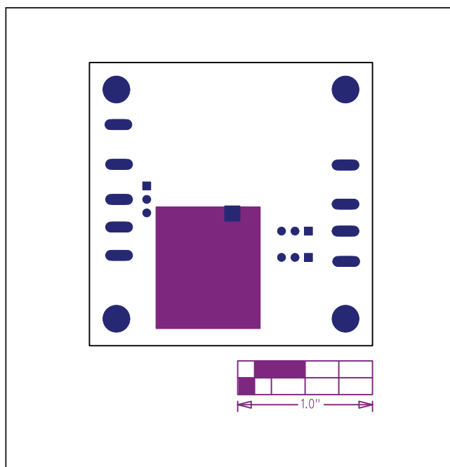
Figure 18. MAX17543 5V Output EV Kit Component Placement Guide—Bottom Solder Mask
