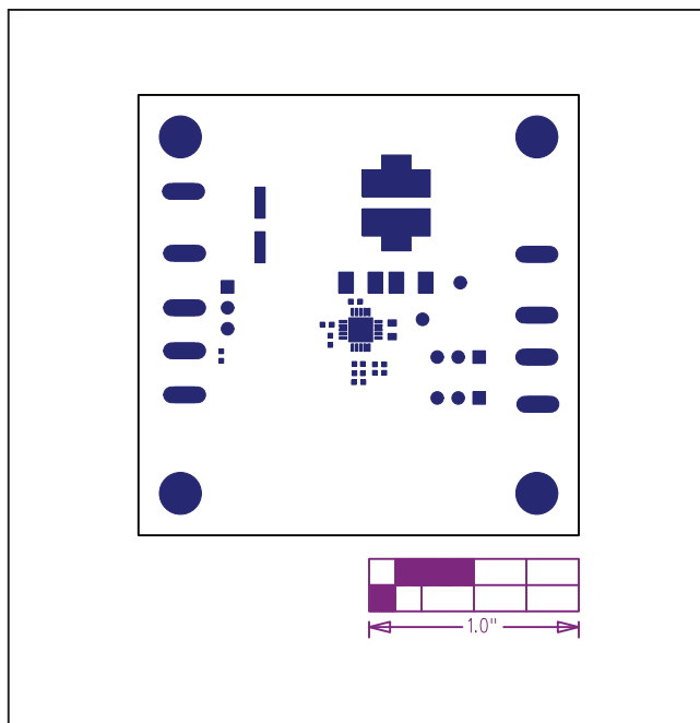
Figure 17. MAX17543 5V Output EV Kit Component Placement Guide—Top Solder Mask
