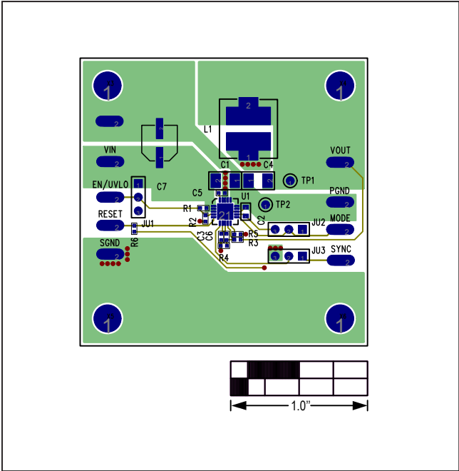
Figure 13. MAX17543 5V Output EV Kit Component Side PCB layout
