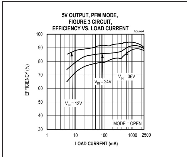
Figure 4. MAX17543 5V Output Efficiency (PFM Mode)
