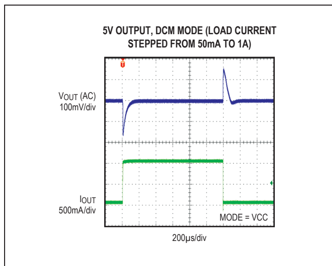
Figure 9. MAX17543 5V Output, 50mA to 1A Load Transient (DCM Mode)
