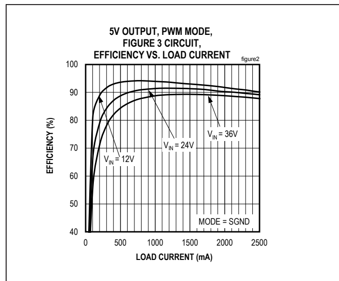
Figure 2. MAX17543 5V Output Efficiency (PWM Mode)
