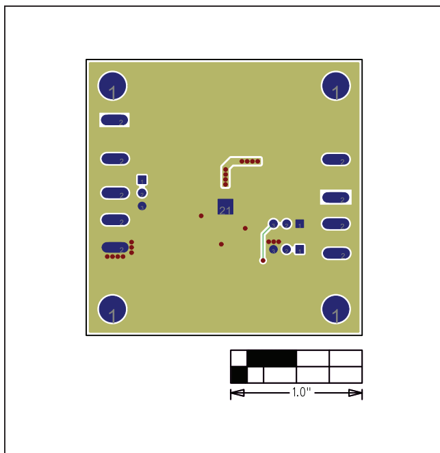
Figure 16. MAX17543 5V Output EV Kit PCB Layout—Solder Side
