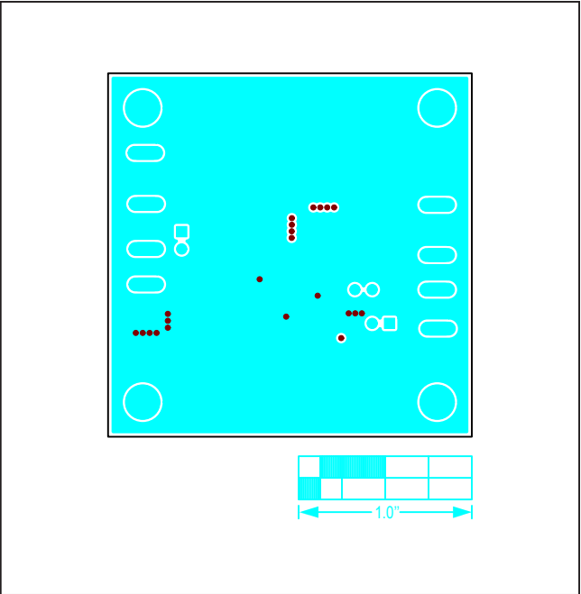
Figure 14. MAX17543 5V Output EV Kit PCB Layout—Inner Layer 1
