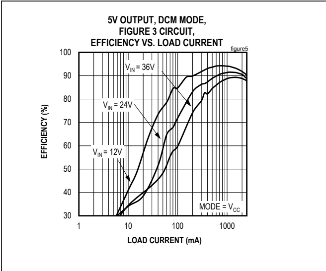
Figure 5. MAX17543 5V Output Efficiency (DCM Mode)
