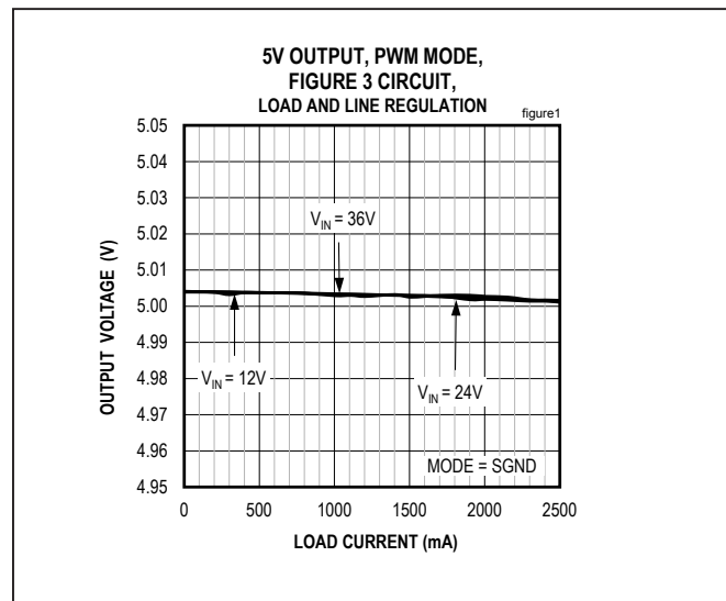
Figure 1. MAX17543 5V Output Load and Line Regulation (PWM Mode)
