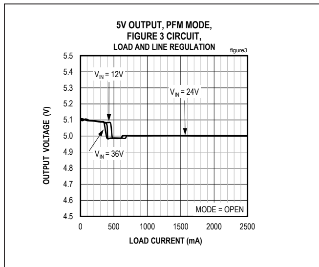
Figure 3. MAX17543 5V Output Load and Line Regulation (PFM Mode)
