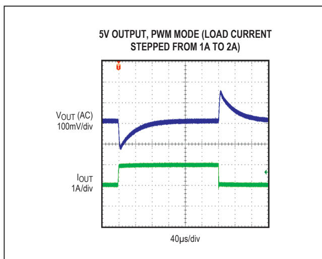
Figure 10. MAX17543 5V Output, 1A to 2A Load Transient
