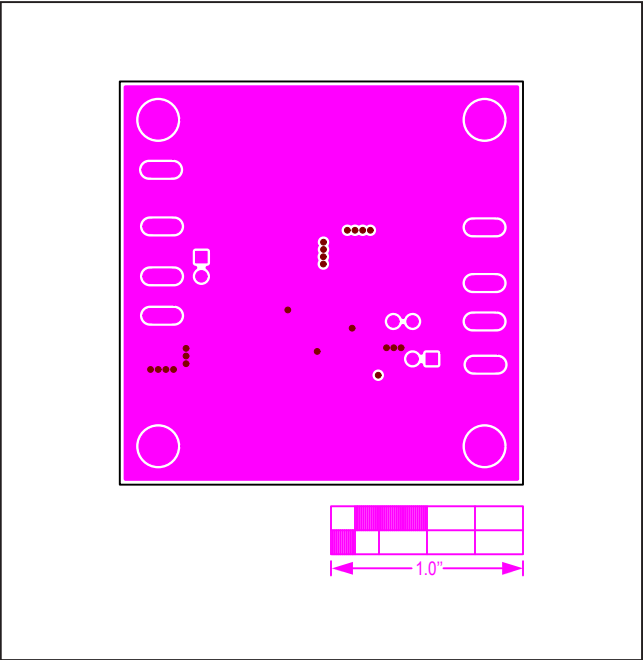
Figure 15. MAX17543 5V Output EV Kit PCB Layout—Inner Layer 2
