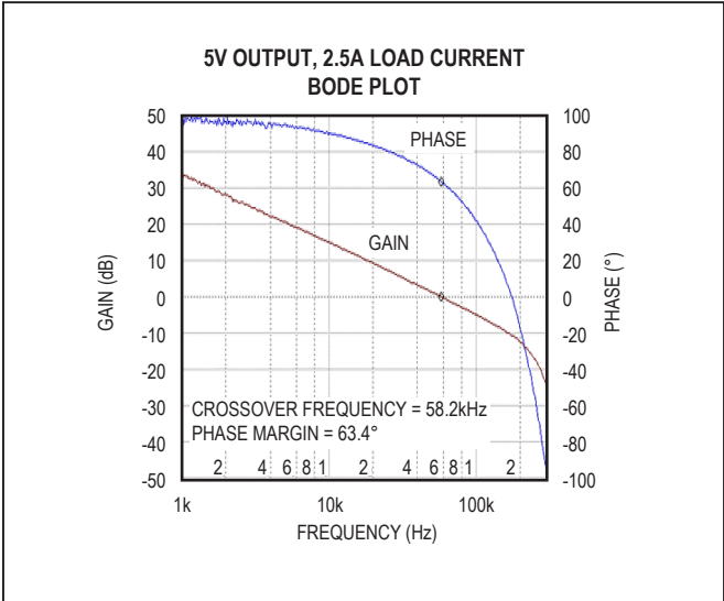
Figure 6. MAX17543 5V Output Full Load Bode Plot ( V_{IN} = 24V )
