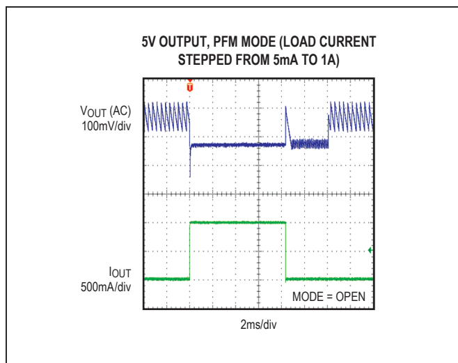
Figure 8. MAX17543 5V Output, 5mA to 1A Load Transient (PFM Mode)
