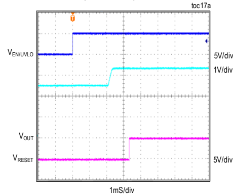
MAX17503S, SOFT-START WITH 2.5V PREBIAS, 3.3V OUTPUT, PWM MODE, FIGURE 4d CIRCUIT
