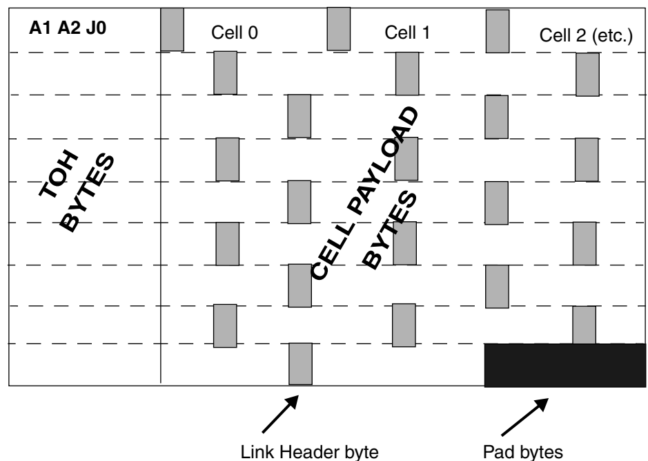
Figure 36. Cell Mapping in SONET Frame
