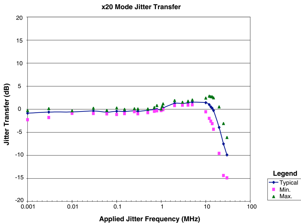
Figure 2-16. Jitter Transfer x20 Mode
