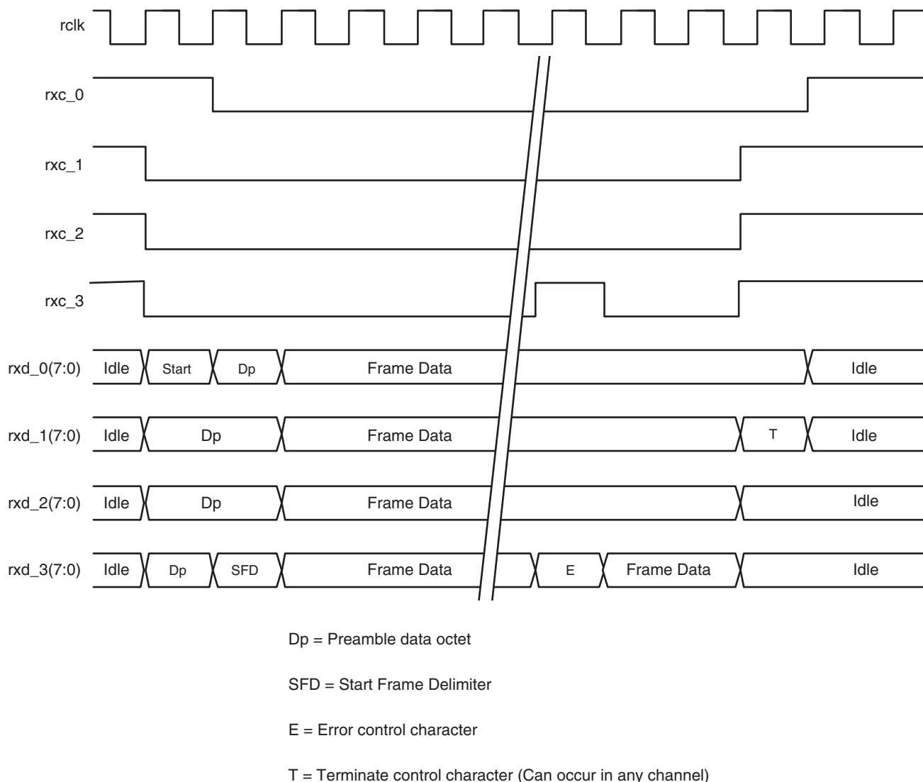
Figure 7-9. XAUI Receive XGMII Interface Signals (Data Error Condition)
