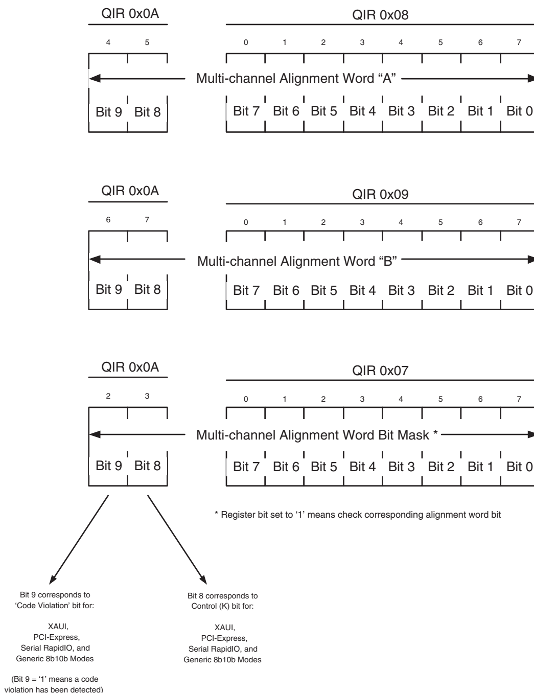
Figure 11-3. Multi-channel Word Alignment Registers for Packet Protocols
