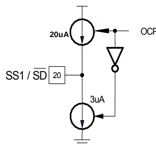
Fig. 8: 3uA current source for discharging soft-start capacitor during hiccup
