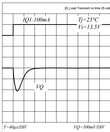
Load Transient Response Peak Voltage dV_Q
