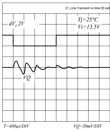
Line Transient Response Peak Voltage dV_Q
