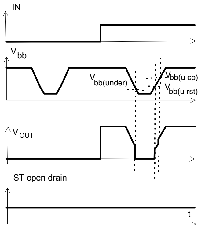
Figure 6a: Undervoltage:
