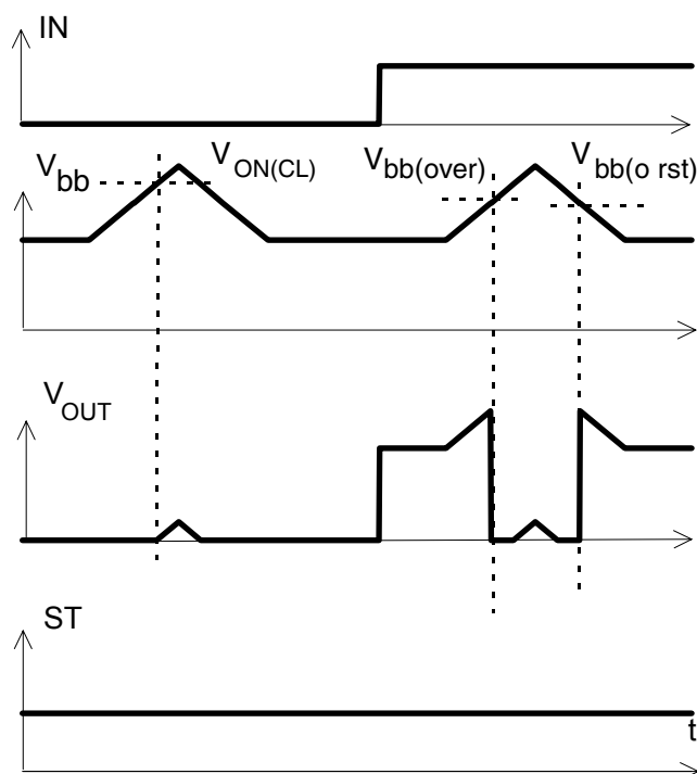
Figure 7a: Overvoltage:
