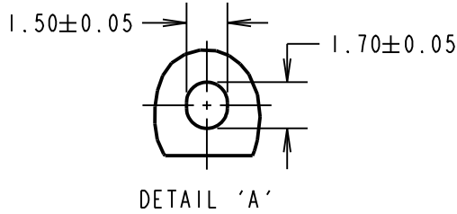
REEL DETAILS
