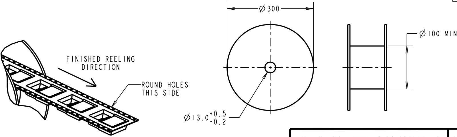
REEL DETAILS
