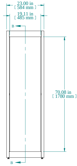
FRONT VIEW
