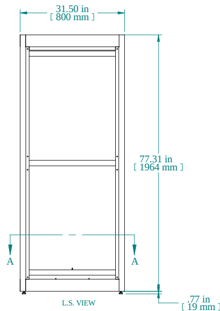
L.S. VIEW
