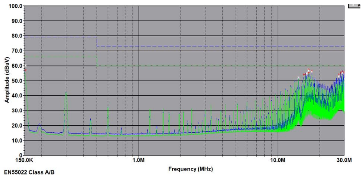
Figure 24. EMC Consideration
