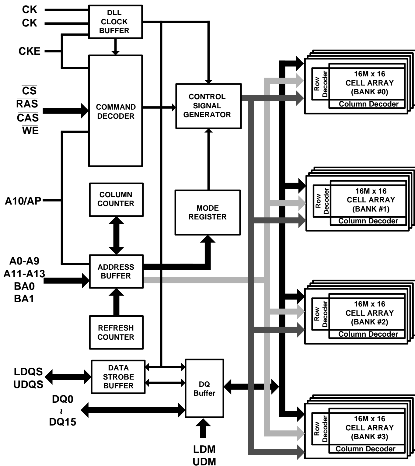
Figure 2. Block Diagram
