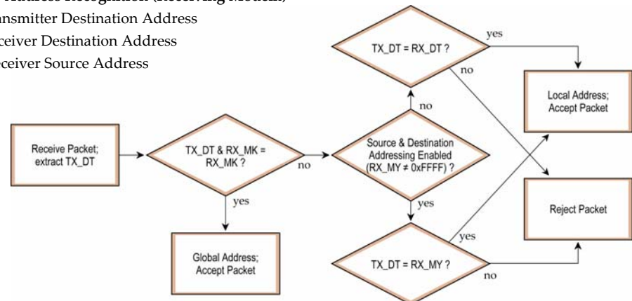
Figure 5-03. Address Recognition (Receiving Modem)
