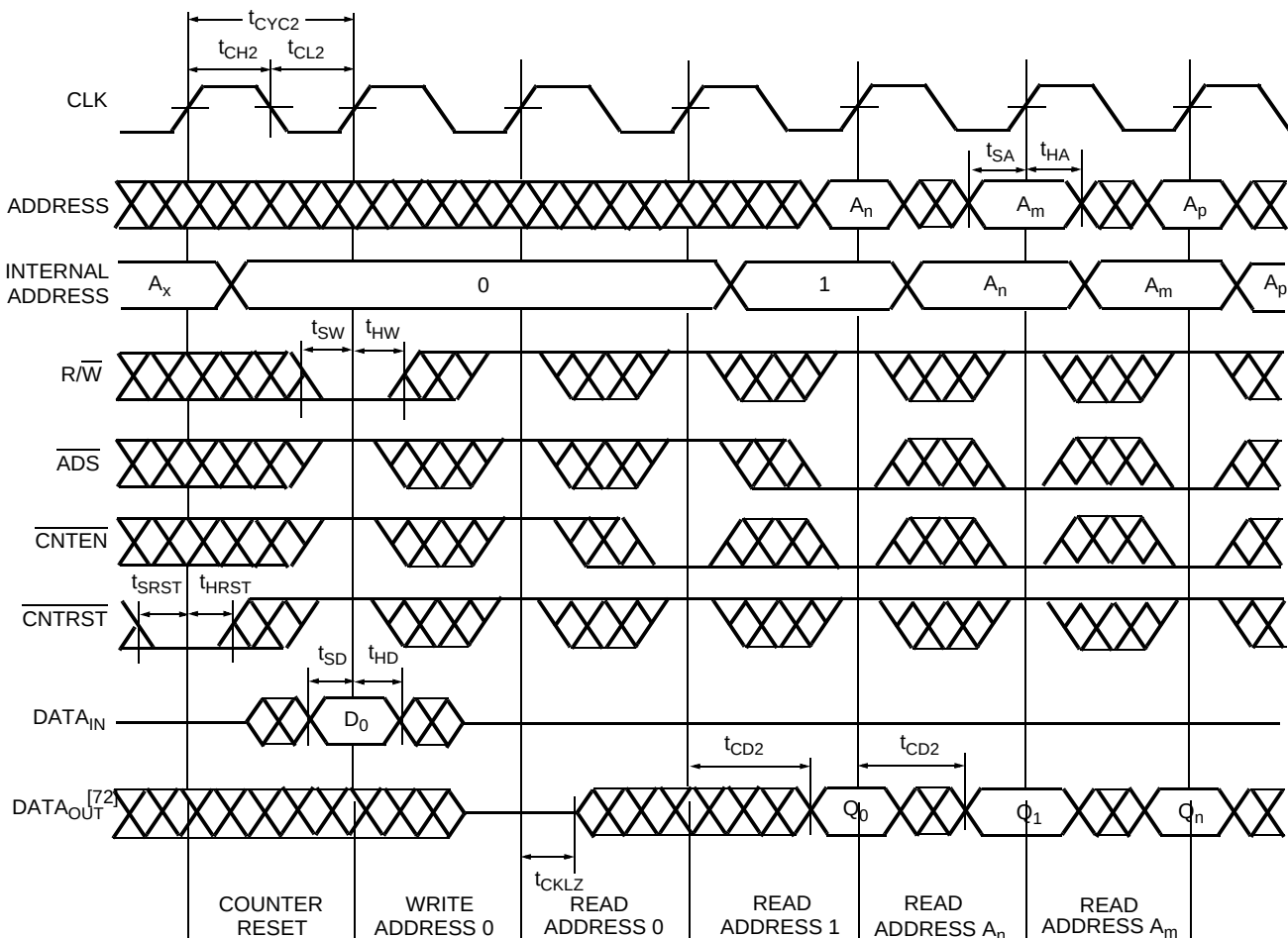
Figure 11. Counter Reset [59, 60]
