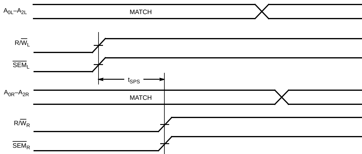
Figure 10. Timing Diagram of Semaphore Contention (CY7C1342 Only) [21, 22, 23]
