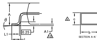
DETAIL A
