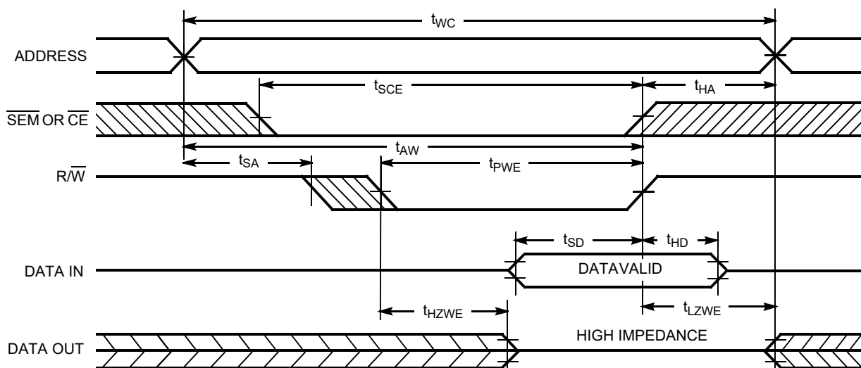
Figure 8. Write Cycle No. 2 ( \text{R}/\overline{\text{W}} Three-state Data I/Os (Either Port)) [20, 22, 23]
