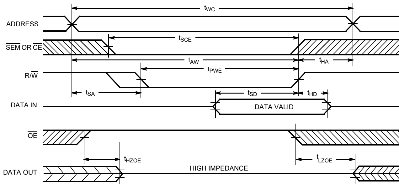
Figure 8. Write Cycle No. 2 ( \text{R}/\overline{\text{W}} Three-state Data I/Os (Either Port)) [20, 22, 23]
